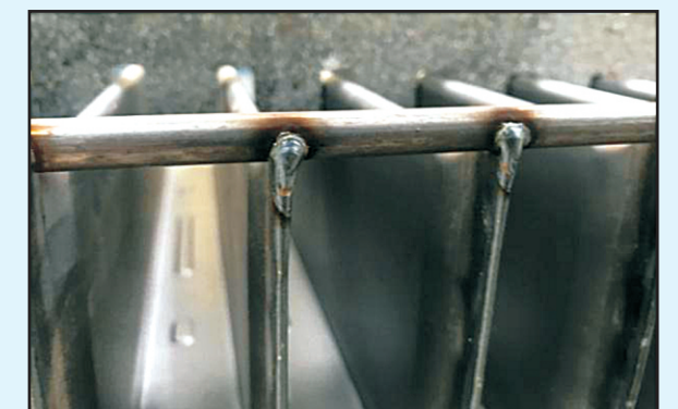
AUTOMATIC STIFFENER ROD WELDING
